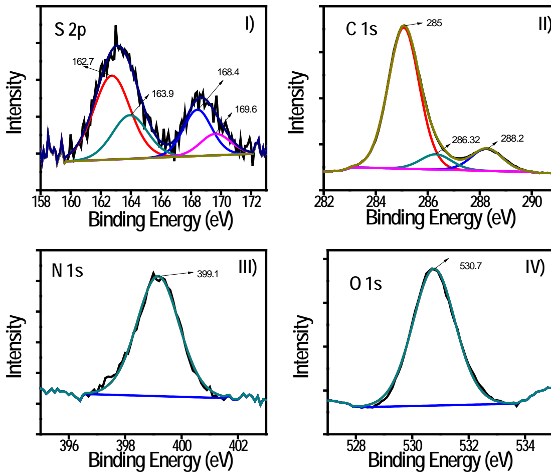
Fig. S7. XPS spectra for individual regions. Spectra were fitted using Casa XPS software.
