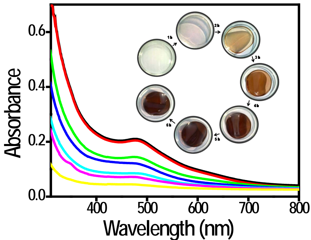
Fig. S4. Time dependent UV/Vis spectra during Ag@SG cluster evaluation. Corresponding photographs are shown in inset.
