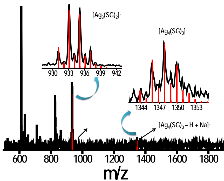
Fig. S9. ESI mass spectrum of as-synthesized cluster in negative mode. Inset shows some fragments with good isotope distribution.
