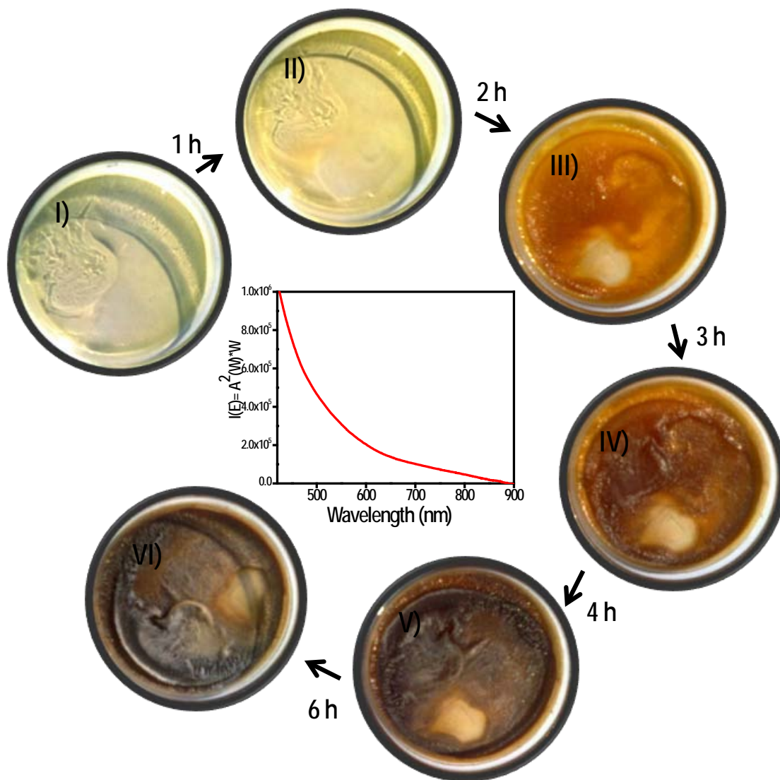
Fig. 17. Polymerized acrylamide gel along with Ag(I)cysteine. I) to VI) are different periods of exposure of sample I) to sunlight. Inset is the UV/Vis spectrum of Ag@cysteine clusters extracted from sample VI).
