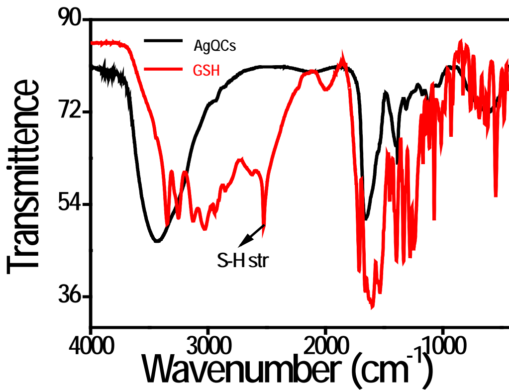
Fig. S8. Comparative IR spectra of AgQCs and GSH. The absence of band at 2552 cm -1 confirms the attachment of glutathione to the cluster core.
