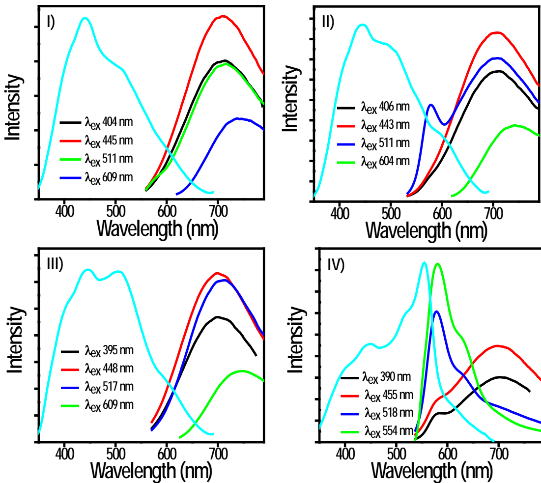
Fig. S10. Excitation and emission spectra of C R (I), C Y (II), C G (III) and C B (IV).
