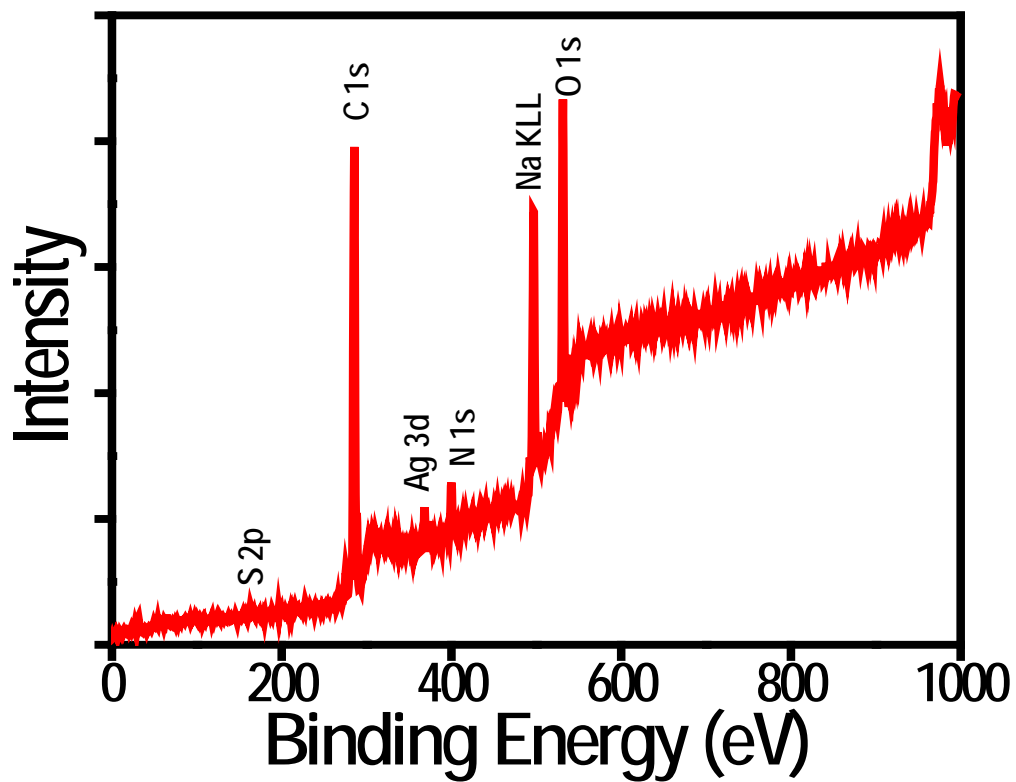
Fig. S6. XPS survey spectrum of the as-synthesized cluster. Individual peaks are labeled.
