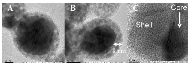
Fig. 2 TEM images of Ag-PBT showing clearly the core and the shell. The shell thickness was found to be 8 nm (Fig. 2B). Fig. 2C shows the Moiré fringes in the core region of the particle as a result of the exposure of various crystallographic planes to the electron beam.
