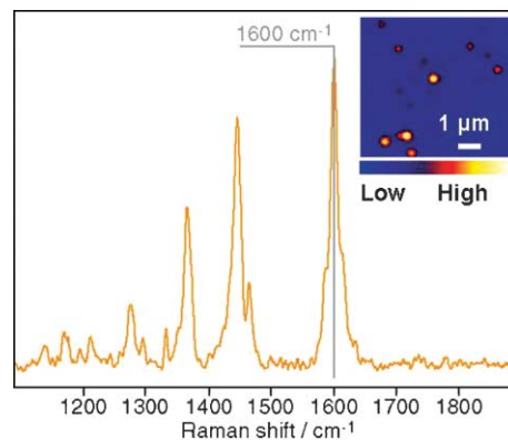
Fig. 5 SERRS spectrum of the polymer on the silver nanoparticle using 532\text{ nm} excitation. Inset shows the Raman image of Ag-PBT aggregates using the intensity of the 1600\text{ cm}^{-1} band.
