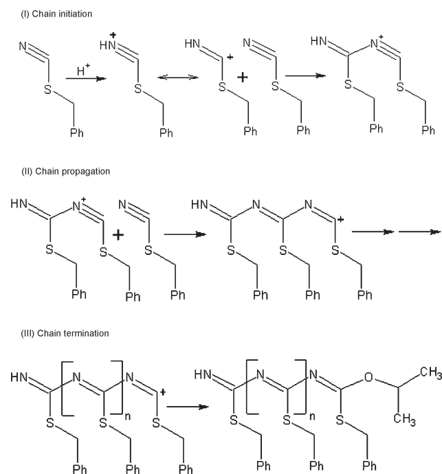
Scheme 1 Probable mechanism for the formation of the polymer.
