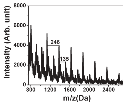
Fig. 6 LDI mass spectrum of Ag-PBT. The two distinct series observed are indicated.
