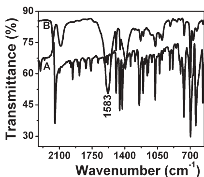
Fig. 4 FT-IR spectra of benzylthiocyanate (curve A) and Ag-PBT (curve B).
