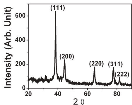
Fig. 3 X-ray diffractogram of Ag-PBT.
