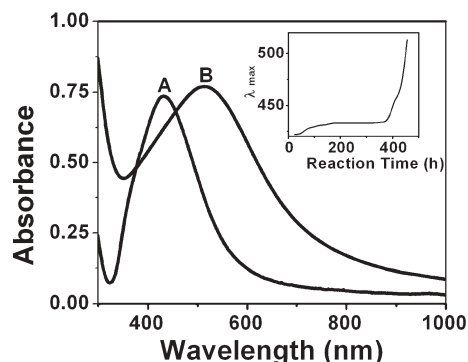
Fig. 1 UV-vis absorption spectrum of Ag-citrate in water (A) and Ag-PBT in isopropyl alcohol (B). The inset shows the position of the surface plasmon band as a function of the reaction time.
