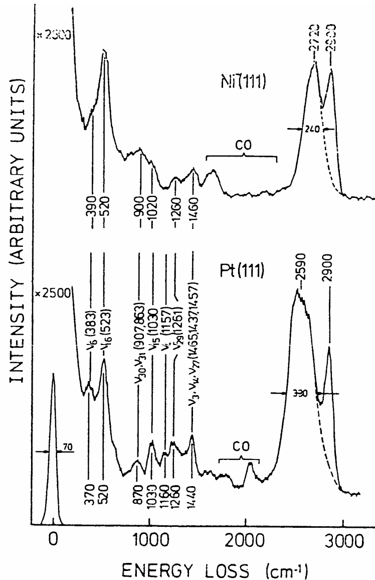
Fig. 6.19 Spectrum of cyclohexane ( \text{C}_6\text{H}_{12} ) adsorbed on Ni(111) and Pt(111) at T = 140^\circ\text{K} ([71] used with permission). All vibrations can be assigned to the A_{1g} , A_{2g} , E_g , and E_u modes of \text{C}_6\text{H}_{12} . Using the dipole selection rule and the correlation tables (Table 4.6), this indicates a symmetry C_s . It is therefore likely that cyclohexane assumes a canted position with three hydrogens pointing towards the surface. The hydrogen atoms give rise to the strong broad CH stretching band suggesting hydrogen bonding on the molecule to the surface.
